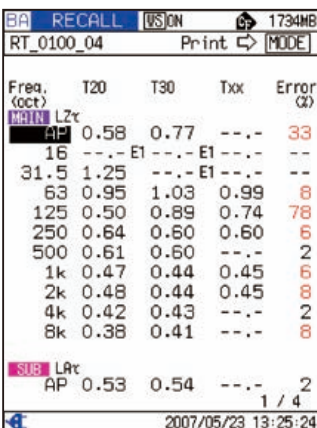
Measured value list of reverberation time
